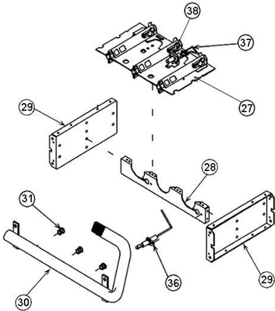
Burner Assembly
